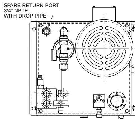
"O" & "S5" OPTION MANIFOLD (P & T BLOCK & D05 SINGLE STATION) SHOWN WITH OPTION "O" RETURN FILTER
