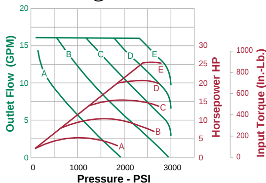
PVP33 @ 1800 RPM
