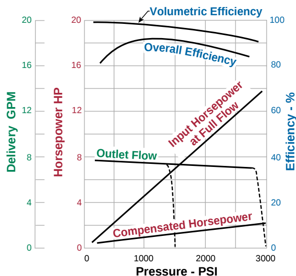
PVP16 @ 1800 RPM
