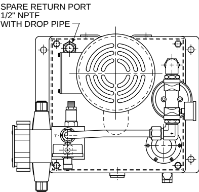
"M3*" OPTION MANIFOLD (MULTI-STATION D03 MANIFOLD) SHOWN WITH OPTION "O" RETURN FILTER
