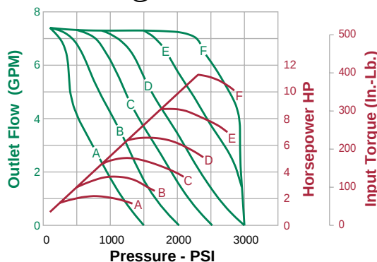
PVP16 @ 1800 RPM
